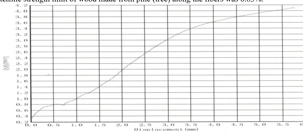
Figure.1 The curve diagram during experimental tensile testing of a wood sample.
